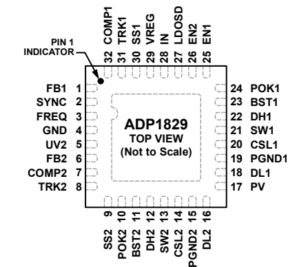
Figure 3. Pin Configuration
