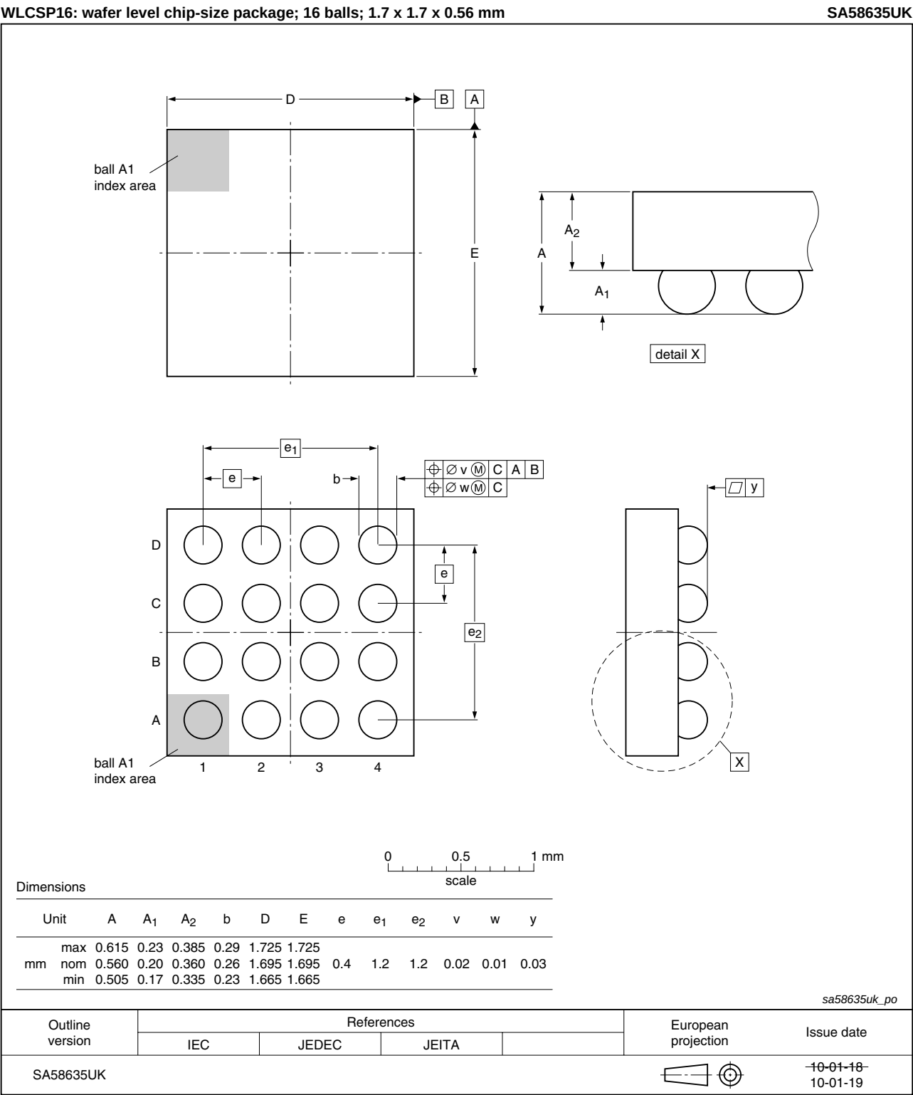
Fig 26. Package outline SA58635UK (WLCSP16)
