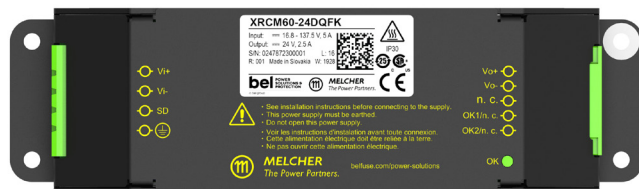
Fig. 14b Pin allocation of RCM60 (K option)
