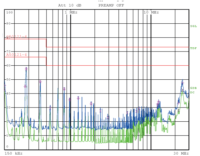
Fig. 9b XRCM60-24: Typ. disturbance voltage at the input ( V_i = 137.5 V, I_{i,nom} , resistive load, quasi peak and average)
