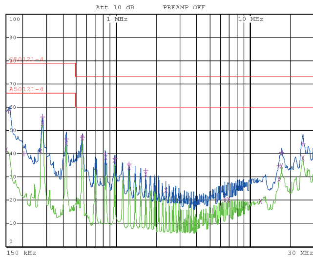
Fig. 9a XRCM60-24: Typ. disturbance voltage at the input ( V_i = 16.8 V, I_{i,nom} , resistive load, quasi peak and average)
