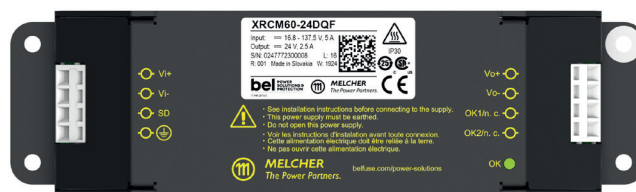
Fig. 13 Pin allocation of RCM60 (standard version)
