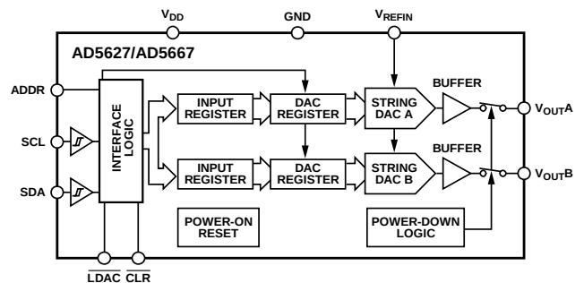
Figure 2. AD5627/AD5667
