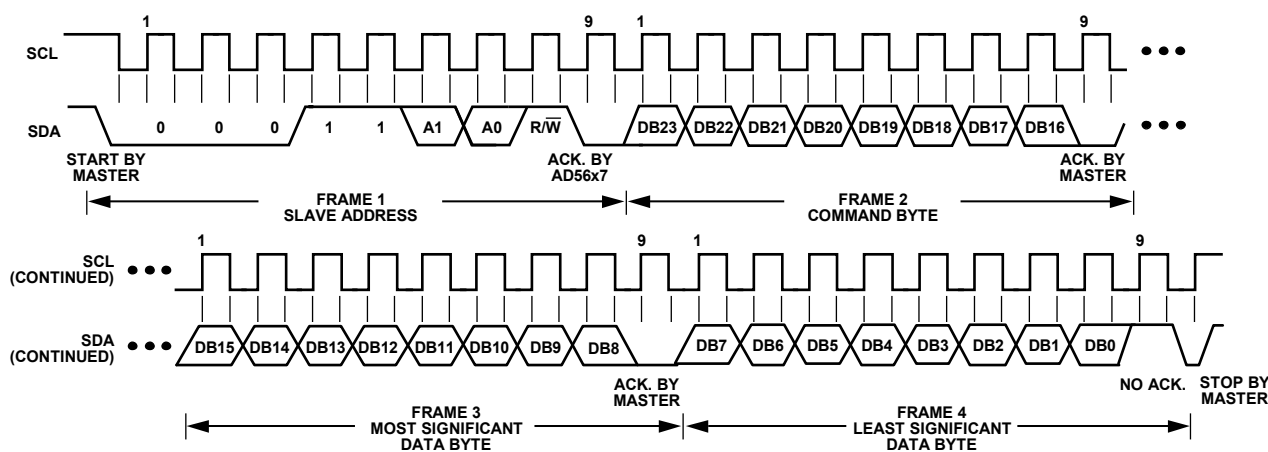
Figure 55. I²C Read Operation
