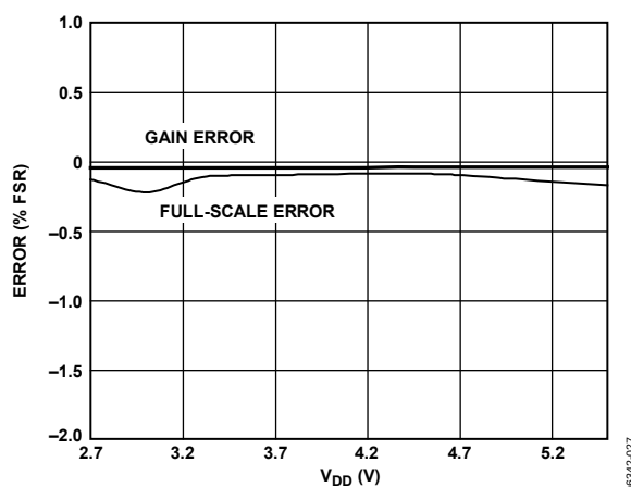
Figure 29. Gain Error and Full-Scale Error vs. Supply
