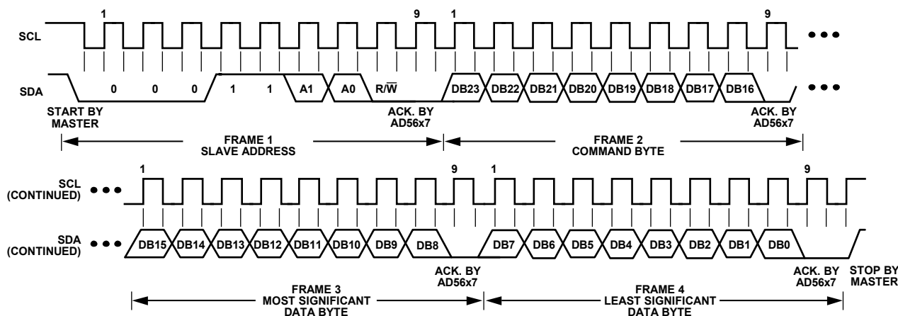
Figure 54. I²C Write Operation
