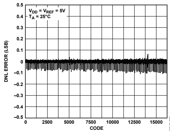
Figure 10. DNL AD5647R, External Reference
