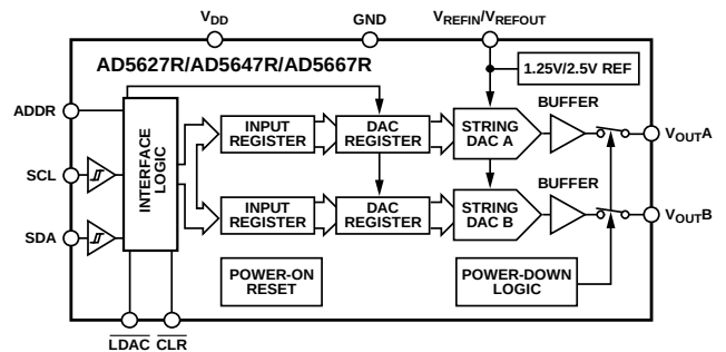
Figure 1. AD5627R/AD5647R/AD5667R
