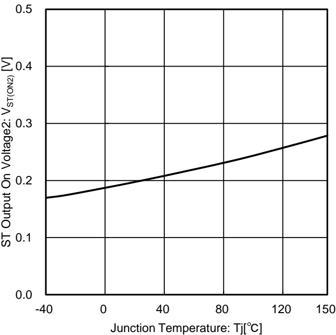
Figure 28. ST Output On Voltage2 vs Junction Temperature
