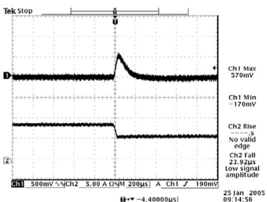
Vout= 12 V 75%-50% Load Transients
