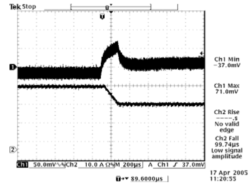
Vout= 1.5 V 75%-50% Load Transients
