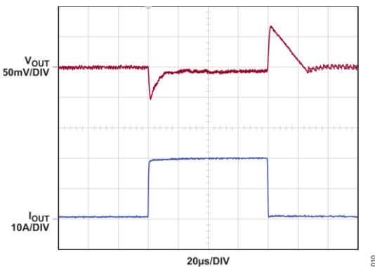
Figure 13. Transient Response, DCM
