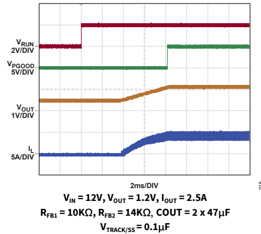
Figure 17. Start-Up Waveform (with Prebiased Output)
