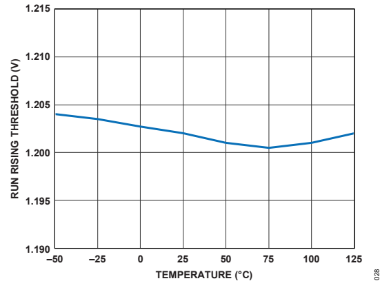
Figure 27. RUN Rising Threshold vs Temperature
