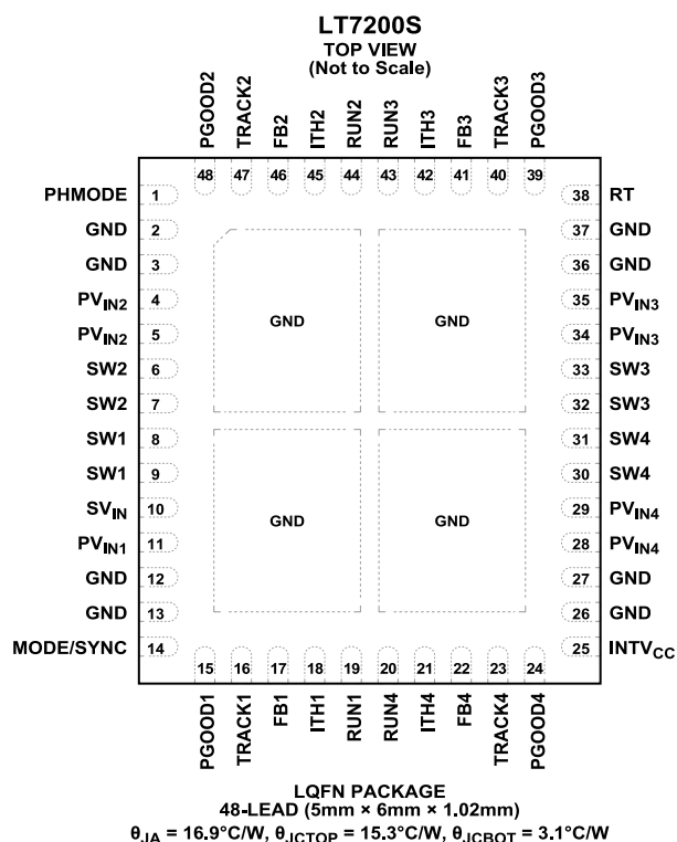
Figure 3. Pin Configurations
