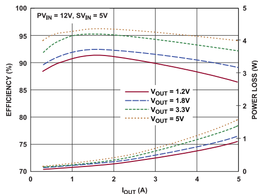
Figure 2. Efficiency and Power Loss (1MHz)
