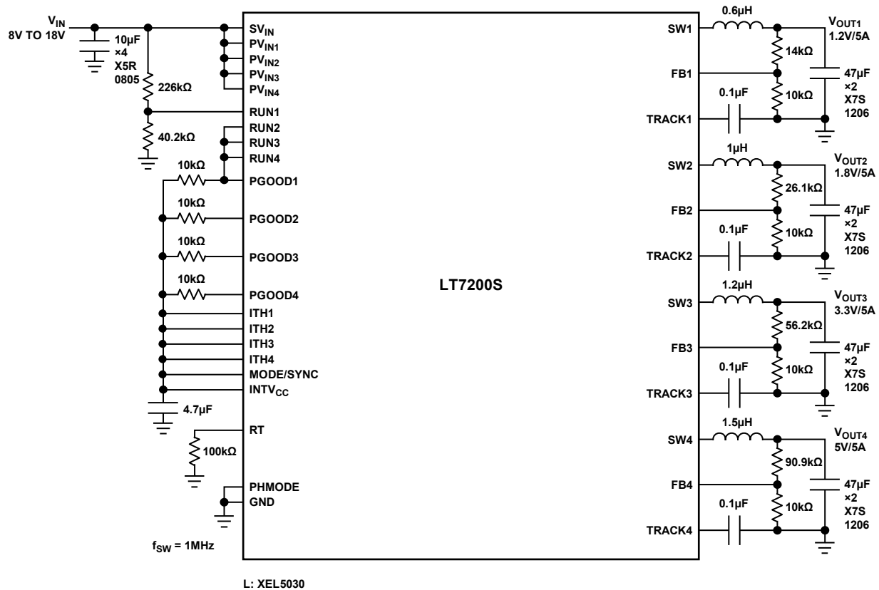
Figure 45. Quad 1.2V/5A, 1.8V/5A, 3.3V/5A, 5V/5A Sequenced Buck Regulator with 8V Input UVLO ( V_{OUT2/3/4} Enabled by PGOOD1/2/3 )
