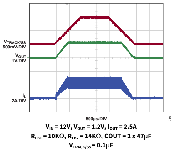
Figure 18. Output Tracking
