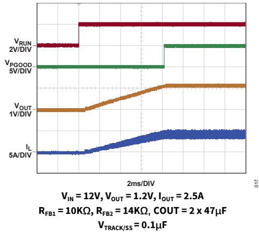
Figure 16. Start-Up Waveform
