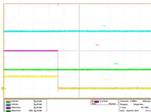
Figure 44: Operation 00, Immediate OFF, 6A load
