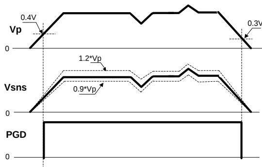
Figure 30: Vp Tracking ( \overline{\text{Track\_En}} = 0\text{V} )
