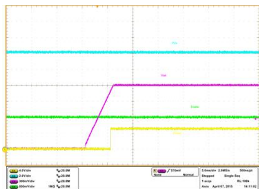
Figure 43: Operation 80, Turn ON without margining, 6A load
