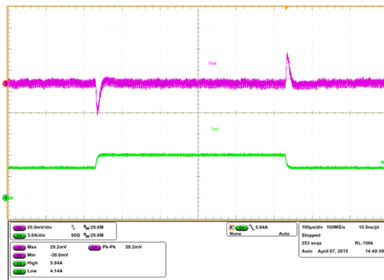
Figure 50: Transient Response, 4.2A to 6A step (2.5A/us)
