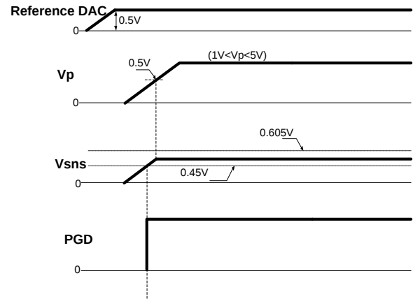
Figure 31: Vp Sequencing (100 kOhm from \overline{\text{Track\_En}} to P1V8)
