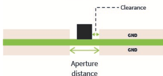
Figure 6 Scenario 1: NFC chip set integrated on the PCB with apertures on both side of the ground planes
