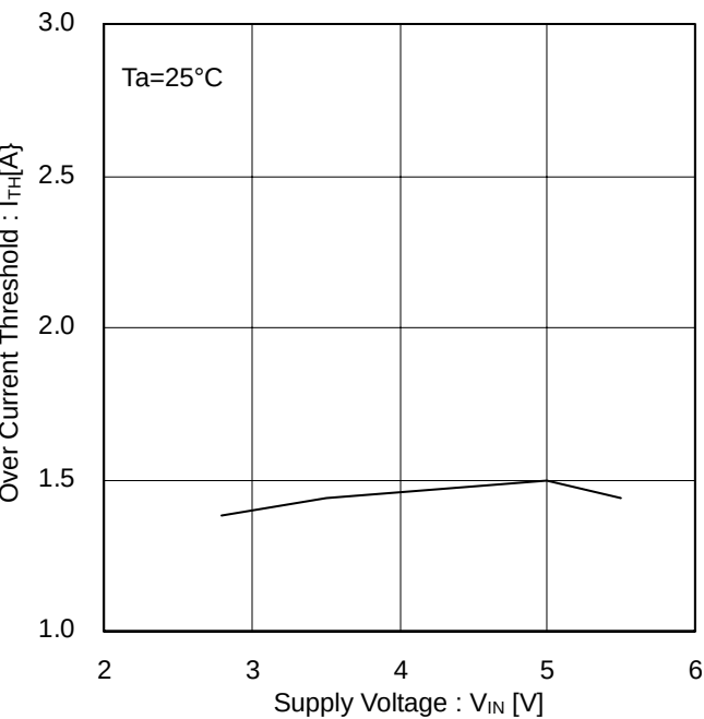
Figure 14. Over-Current Threshold
