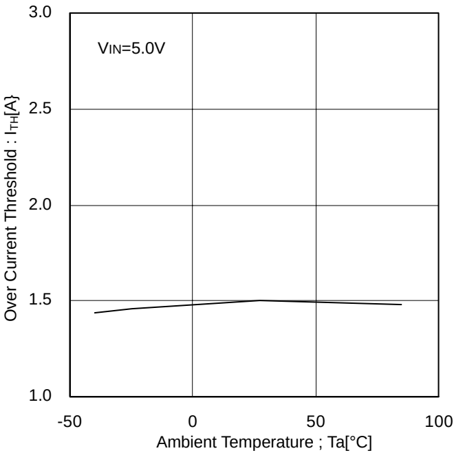
Figure 15. Over-Current Threshold
