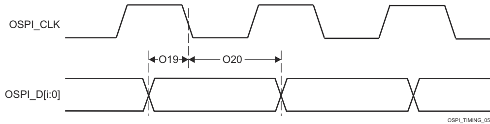
Figure 7-110. OSPI Timing Requirements – SDR, Internal Clock and Internal Pad Loopback Clock
