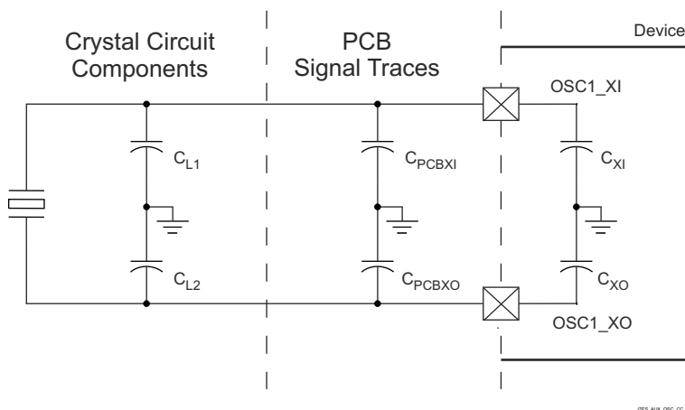
Figure 7-30. Load Capacitance
