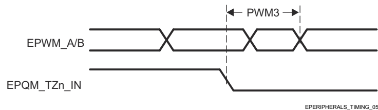
Figure 7-60. EPWM_A/B and ePWM_TZn_IN Forced High/Low Input Timings
