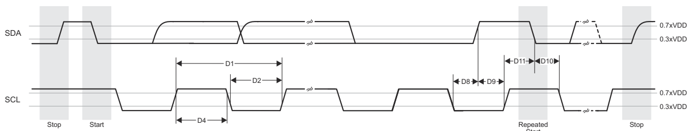
Figure 7-83. I3C Push-Pull Timing Requirements - SDR Mode
