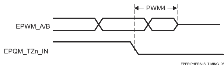
Figure 7-61. EPWM_A/B and ePWM_TZn_IN Hi-Z Input Timings
