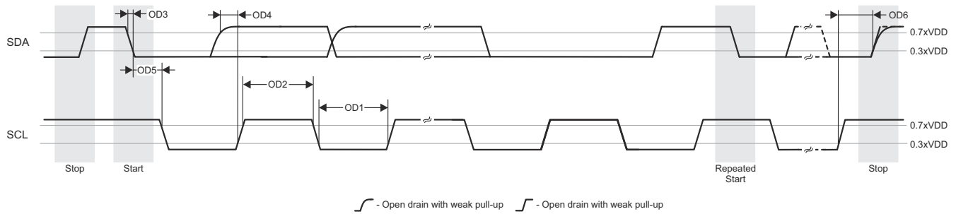
Figure 7-81. I3C Open Drain Timing Requirements
