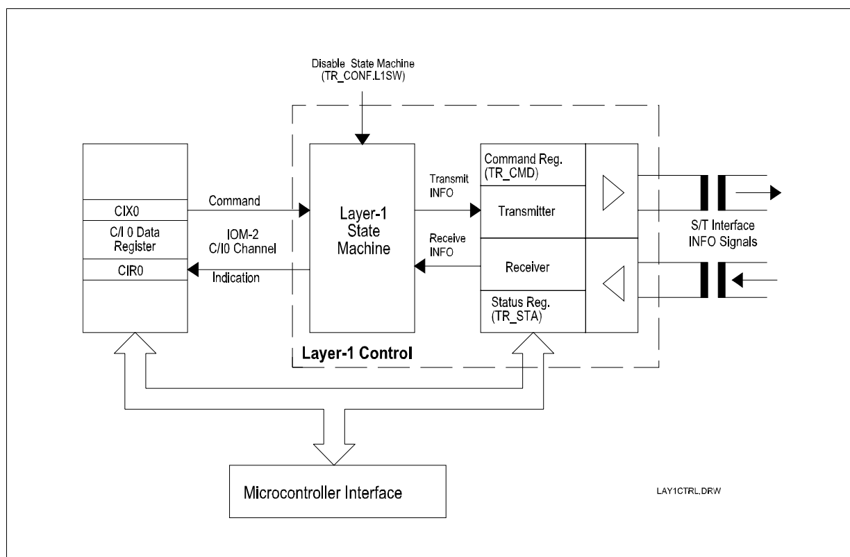
Figure 31 Layer-1 Control
