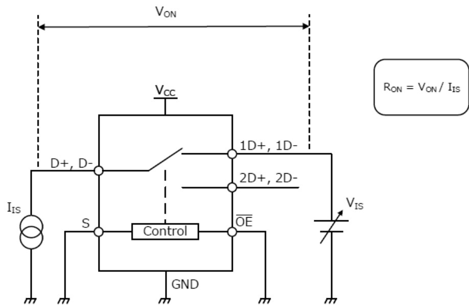
Fig. 11.9 ON-Resistance
