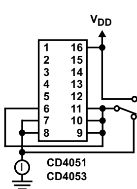
Figure 7-10. Quiescent Device Current
