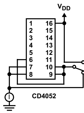
Figure 7-10. Quiescent Device Current
