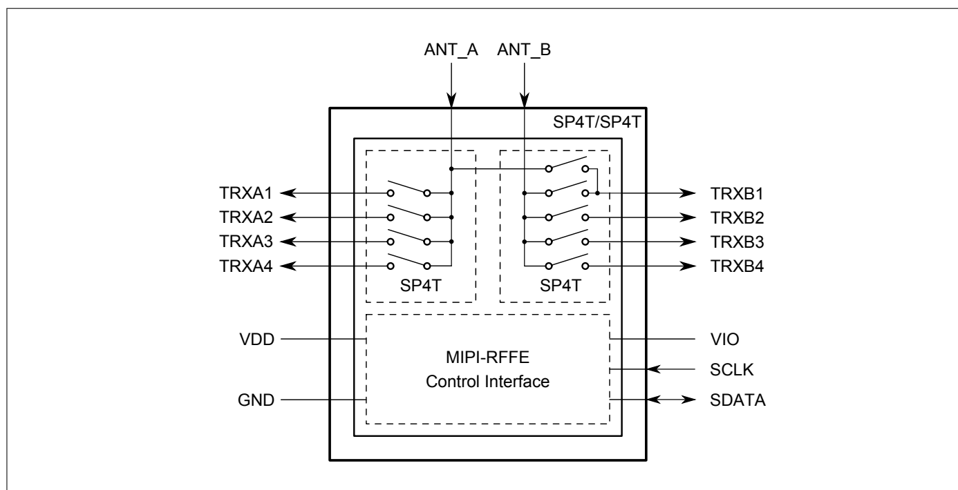
Figure 1: BGSX28MA18 Block diagram
