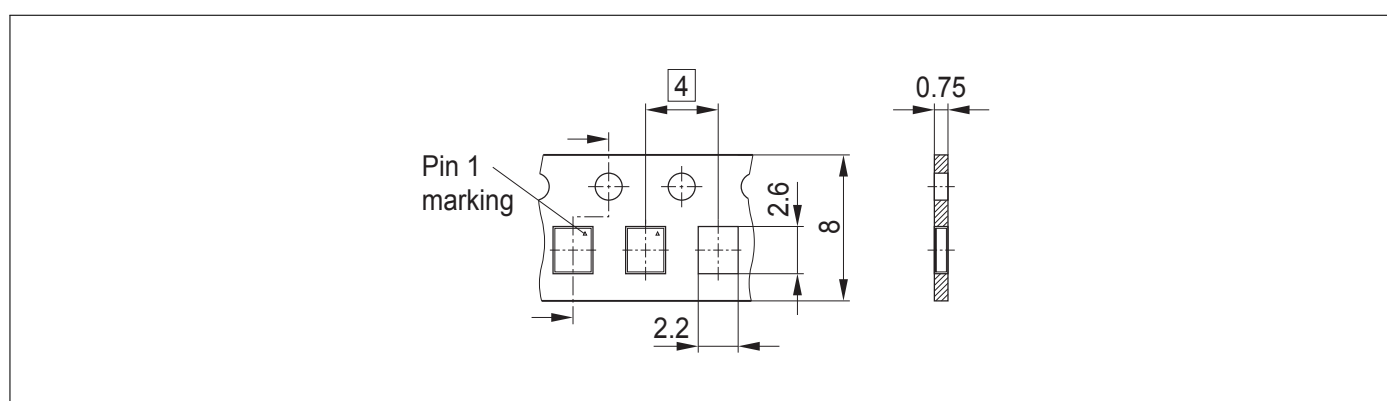
Figure 7: Carrier Tape
