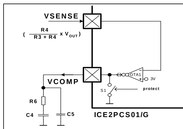
Figure 4 Startup Circuit
