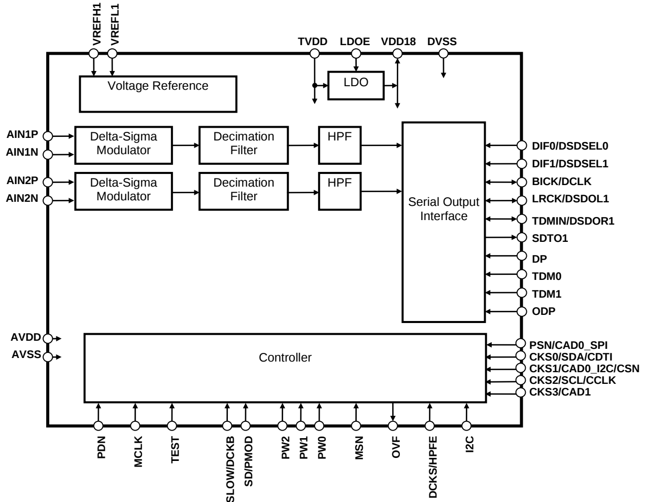
Figure 1. Block Diagram
