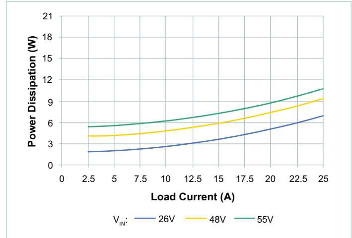
Figure 6 — Power dissipation at 25^\circ\text{C}
