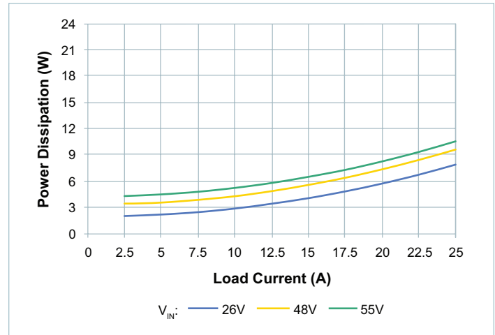
Figure 8 — Power dissipation at 100^\circ\text{C}
