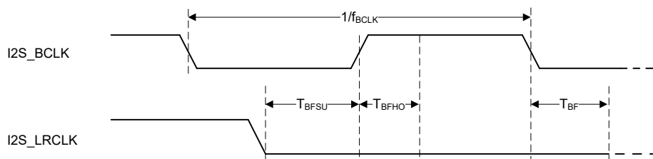
Figure 37. I2S timing specification diagram for clock signal—Peripheral mode
