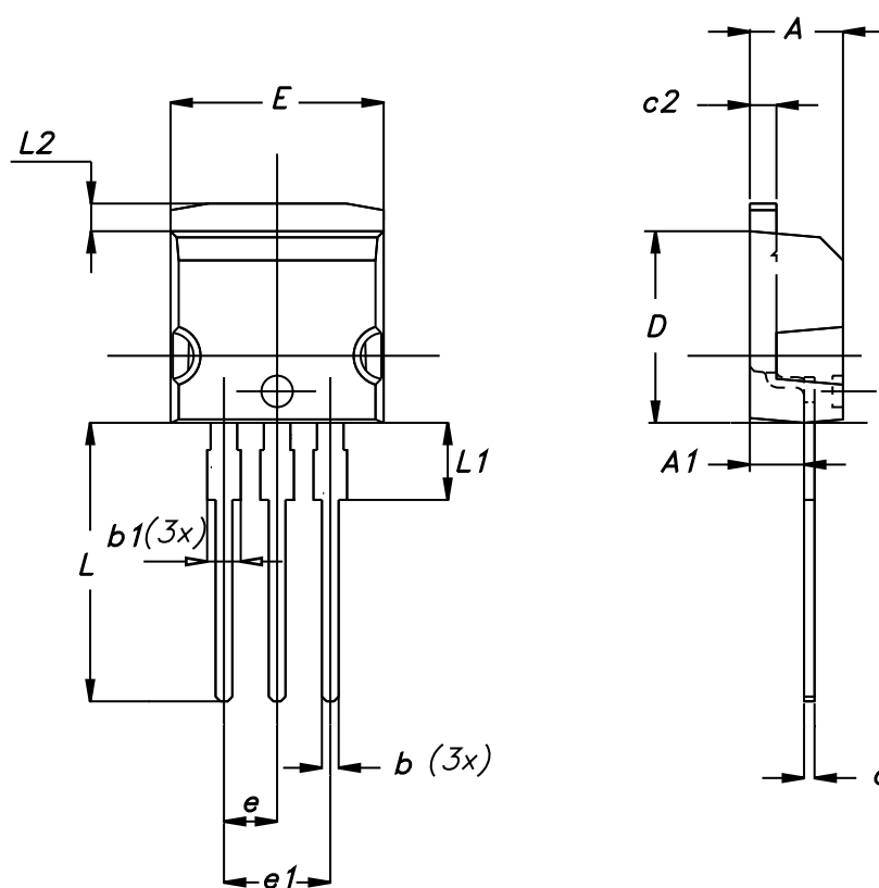
Figure 18. I 2 PAK package outline
