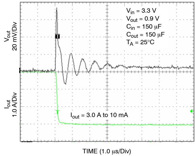
Figure 12. Load Transient Response
