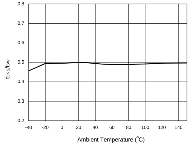
t_{ONS}/t_{SW} Above SUVP vs. Ambient Temperature
