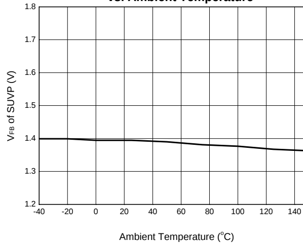
Feedback Voltage of SUVP vs. Ambient Temperature
