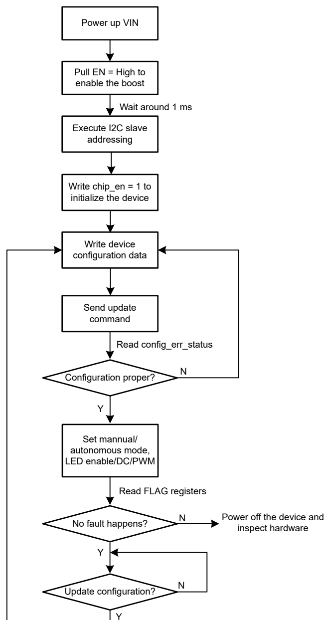
Figure 9-4. Program Procedure
