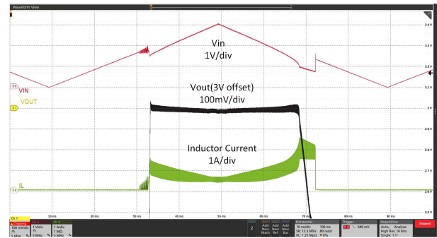
Figure 9-18. Line Sweep
