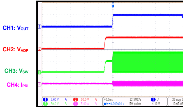
Adapter Start-Up I_{OUT} = 0A
