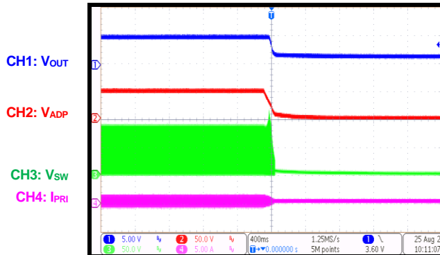
Adapter Shutdown I_{OUT} = 0A
