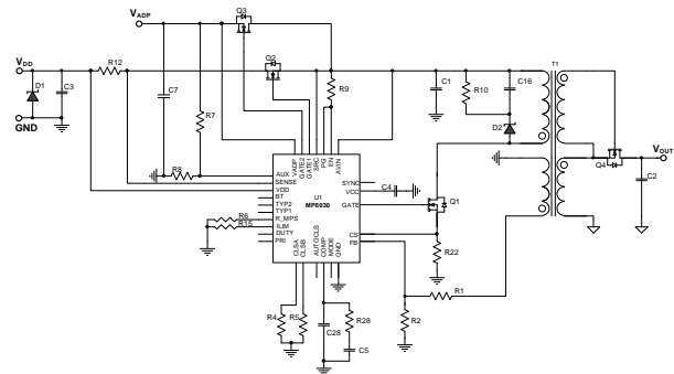
Figure 19: Recommended Flyback Layout
