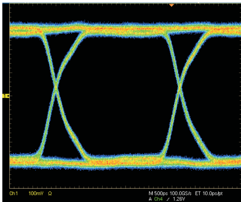
Figure 50. Eye Diagram of LVDS Data Output With Internal Termination
