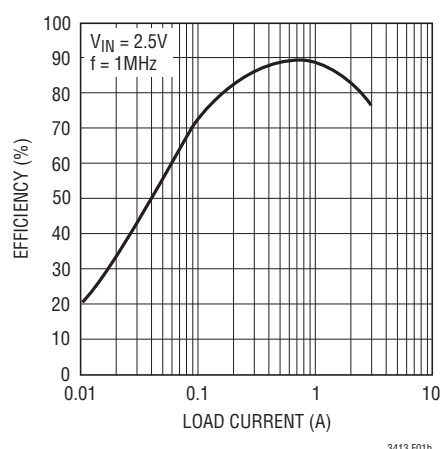
Figure 1b. Efficiency vs Load Current
