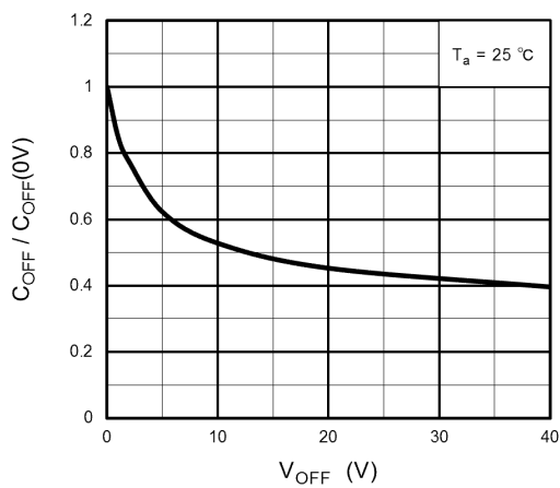
Fig. 12.11 C_{OFF}/C_{OFF}(0V) - V_{OFF}
