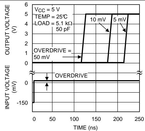
Figure 14. Prop Delay vs Overdrive
