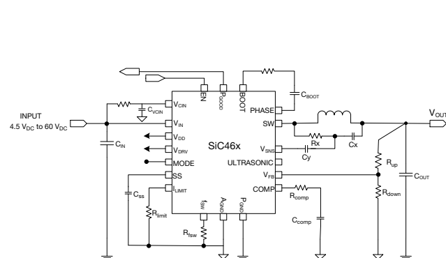
Fig. 1 - Typical Application Circuit for SiC46x
