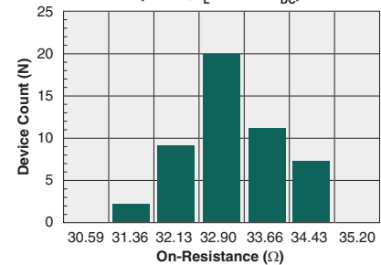
Typical On-Resistance Distribution (N=50, I_L=100\text{mA}_{DC} )
