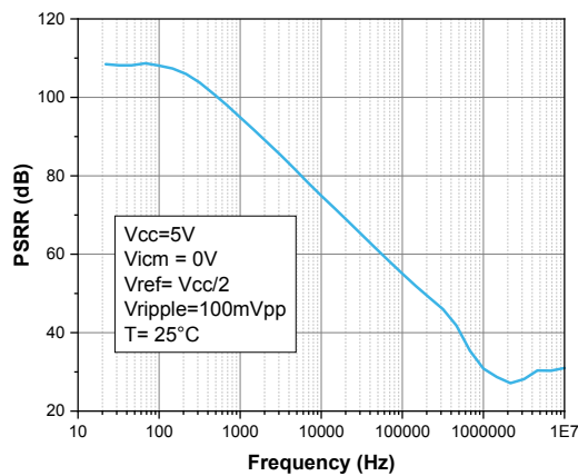
Figure 35. PSRR vs. frequency
