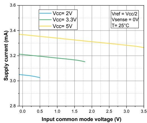
Figure 9. Supply current vs. input common-mode voltage
