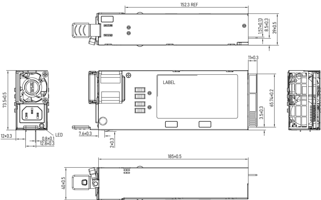
Figure 14. Mechanical Drawing
