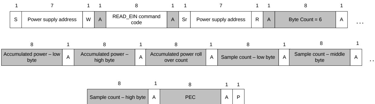
Figure 8. READ_EIN Command
