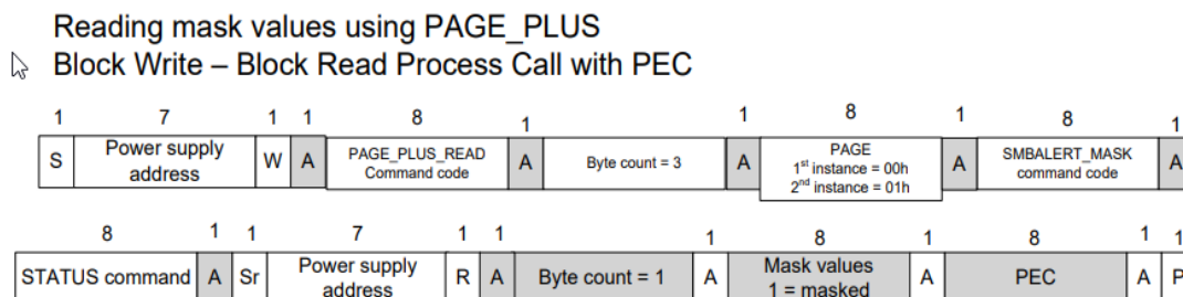
Figure 5. PAGE_PLUS_READ command.
