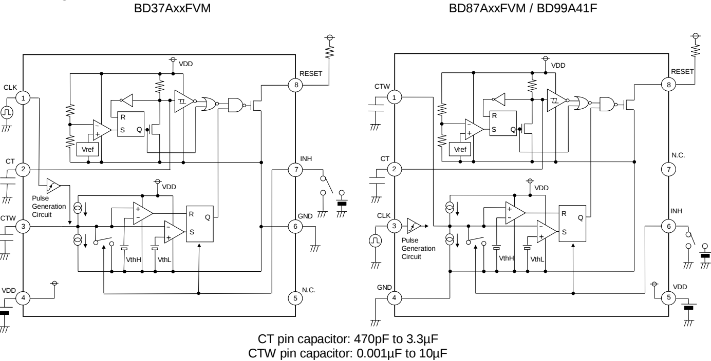
Figure 2. Block Diagrams
