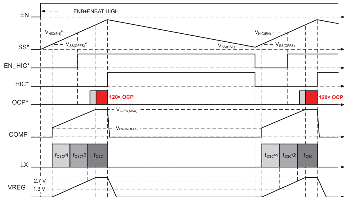
Figure 5: Hiccup Mode Operation with VREG Overloaded ( R_{LOAD} \approx 0.5\text{ }\Omega )
