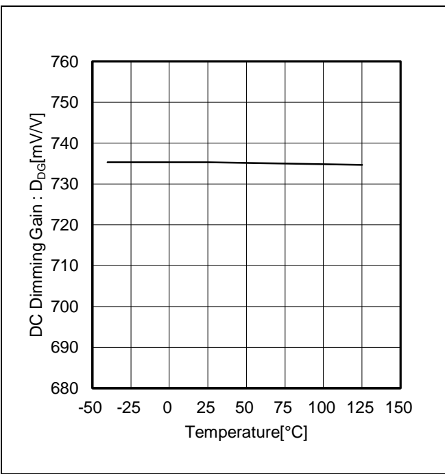
Figure 12. DC Dimming Gain vs Temperature
