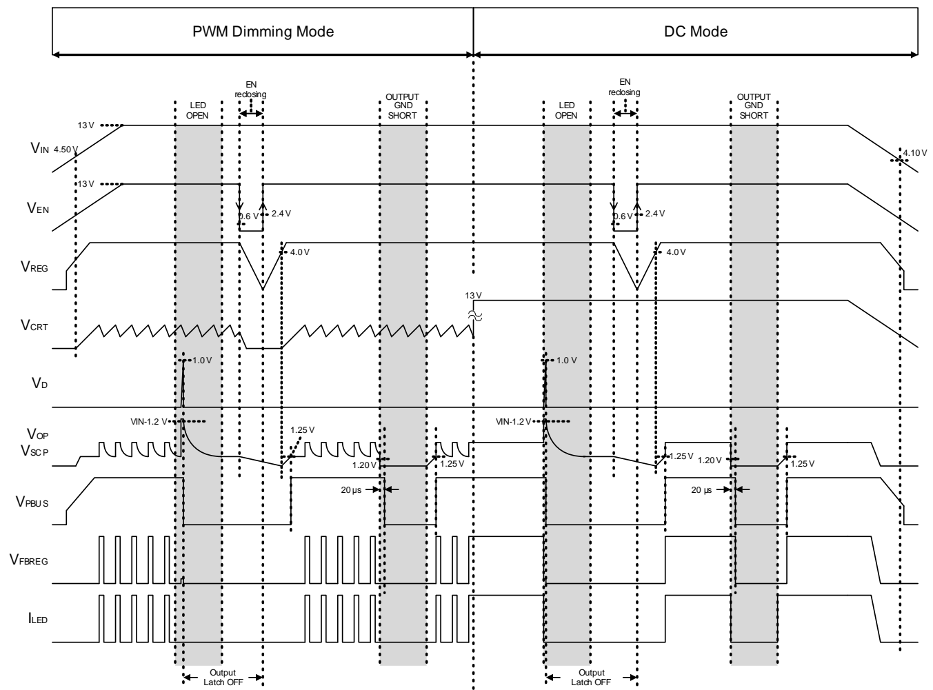
Figure 30. Timing Chart
