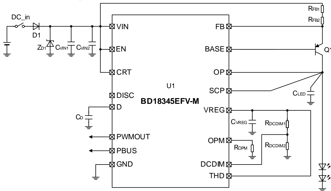
Figure 31. Application Example 1
