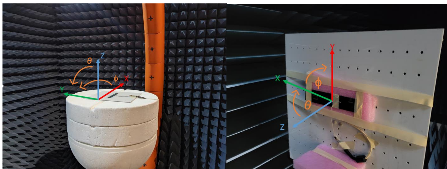
OTA Setup of the FXUB85.07.0150C in the SG24-L Satimo Test System For 600 MHz – 6 GHz Testing
