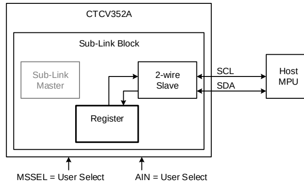
Figure 13. Host to CTCV352A local register access configuration
