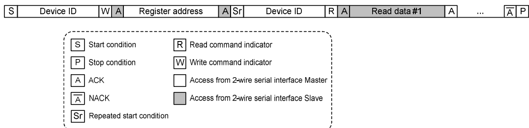
Figure 15. 2-wire serial I/F read to CTCV352A local register protocol
