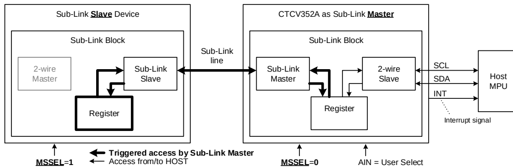
Figure 16. Host MPU to Sub-Link Slave Register via CTCV352A access configuration
