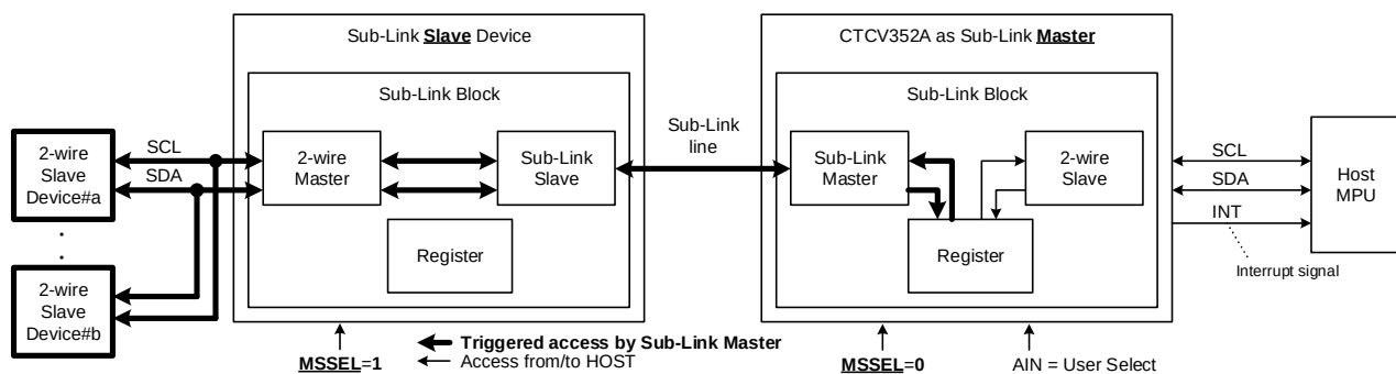
Figure 17. Host MPU to 2-wire slave devices connected to Sub-Link Slave via CTCV352A access configuration
