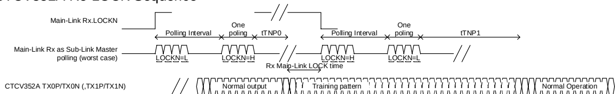
Figure 23. Re-Lock Sequence
