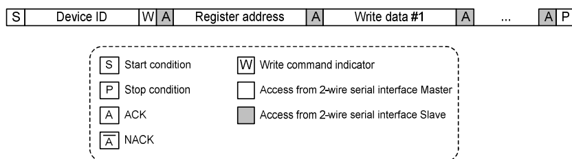
Figure 14. 2-wire serial I/F write to CTCV352A local register protocol
