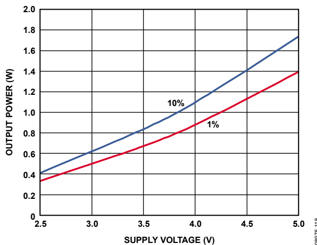
Figure 41. Output Power vs. SPKVDD, 8 Ω + 33 μH (Stereo), Digital In → Speaker Out
