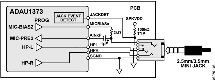
Figure 90. Headphone Jack Detect Option 2
