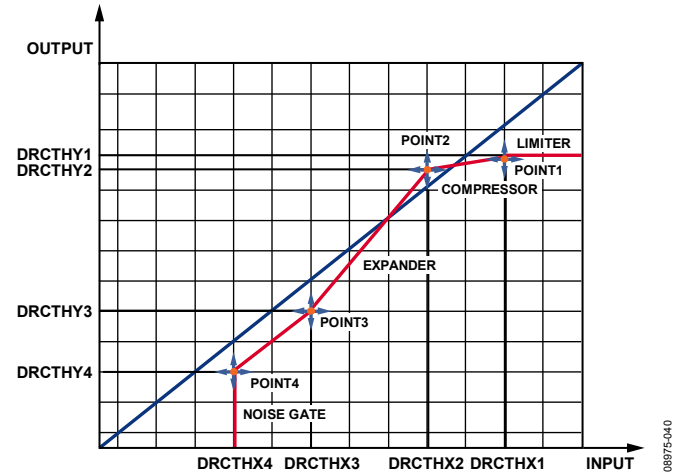
Figure 107. DRC Output vs. Input Plot
