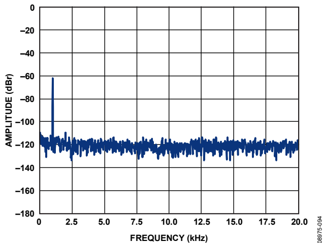
Figure 61. FFT, -60 dBFS, Analog In → Digital Out, PGA Gain = 0 dB
