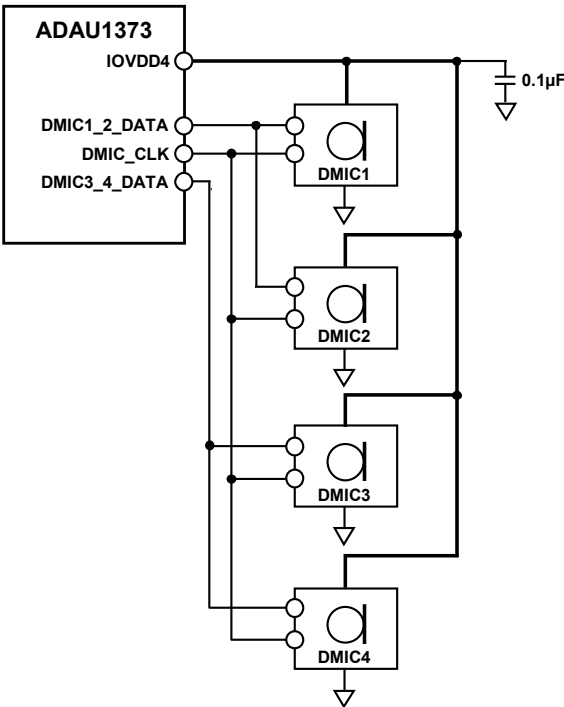
Figure 95. Digital Microphone Connection Diagram for Four Microphones
