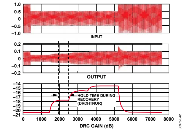
Figure 109. Limiter Dynamic—Working Example Showing Hold Time
