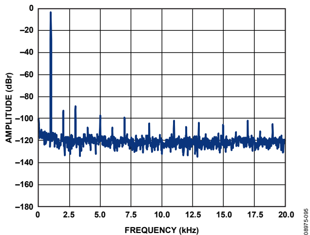
Figure 62. FFT, -1 dBFS, Analog In → Digital Out, PGA Gain = 0 dB
