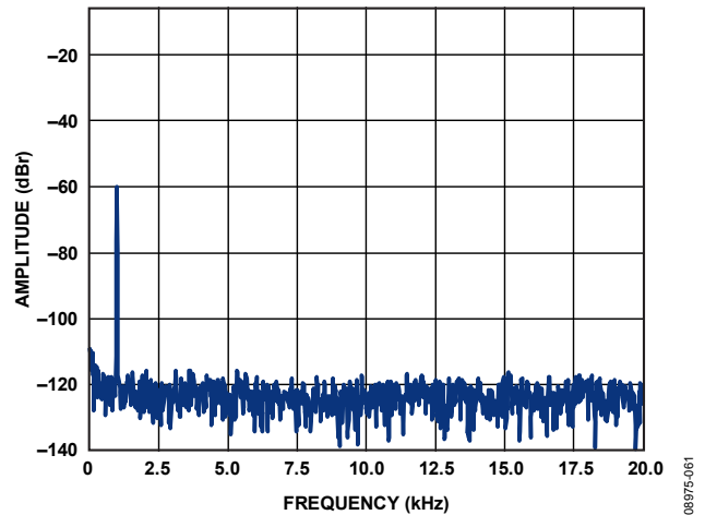
Figure 18. FFT, -60 dBFS, Analog In → Headphone Out
