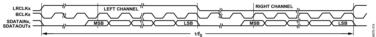
Figure 100. Right-Justified Mode—16 Bits to 24 Bits per Channel
