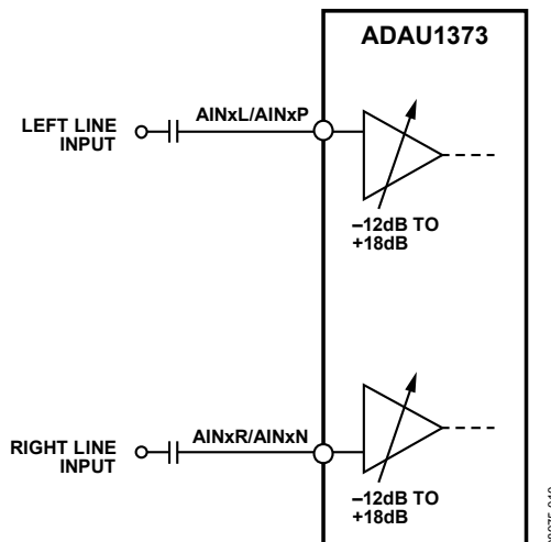
Figure 85. Single-Ended Line Input
