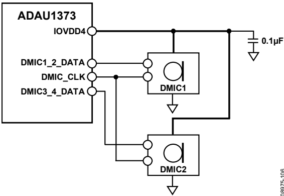
Figure 96. Digital Microphone Connection Diagram for Two Microphones
