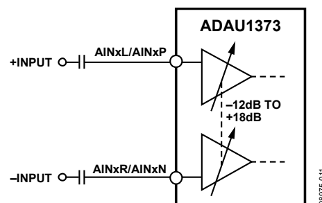
Figure 86. Differential Line Input
