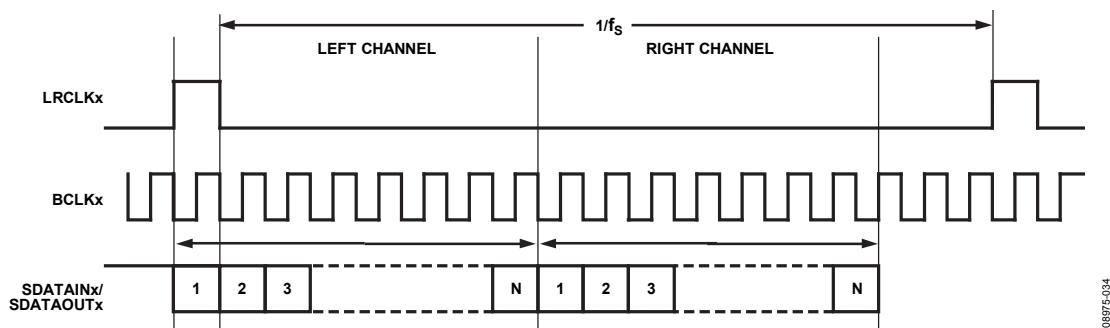
Figure 101. DSP/Pulse Code Modulation (PCM) Mode Audio Interface Submode 1 (SM1), Register 0x44 to Register 0x46, Bit LRPx = 0
