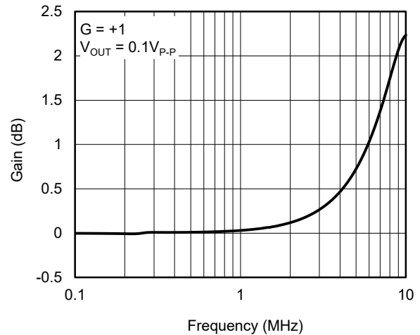
0.1dB Flatness
