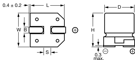
Fig. 2 - Dimensional outline
