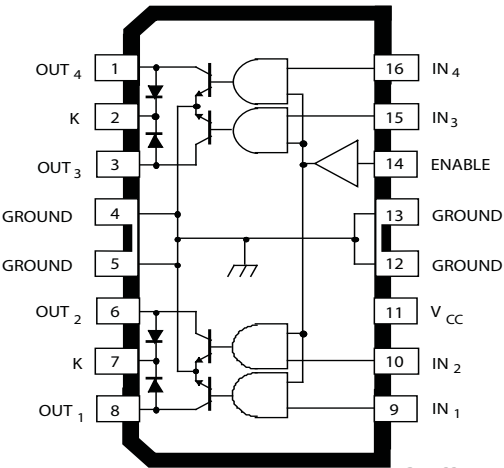
Package LB
