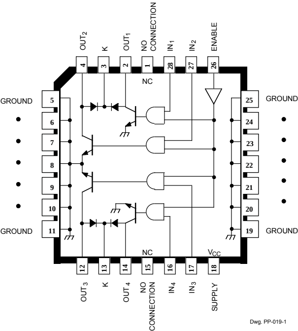
Package EB
