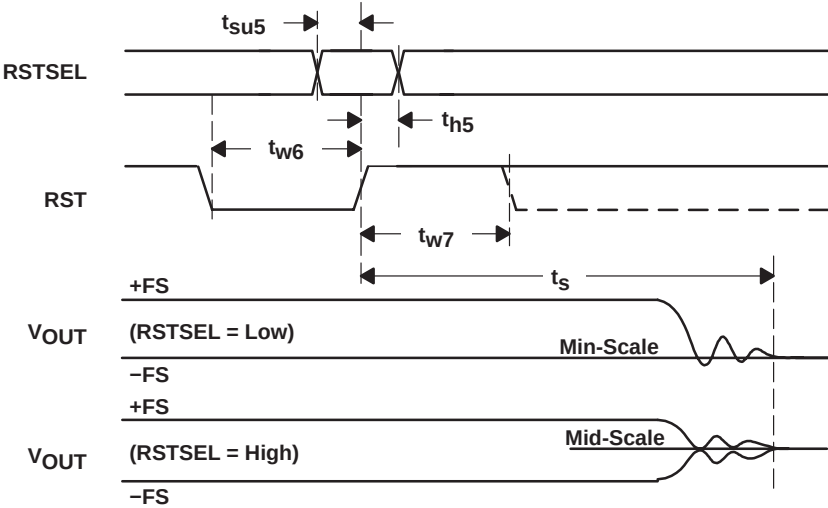
Figure 2. Reset Timing
