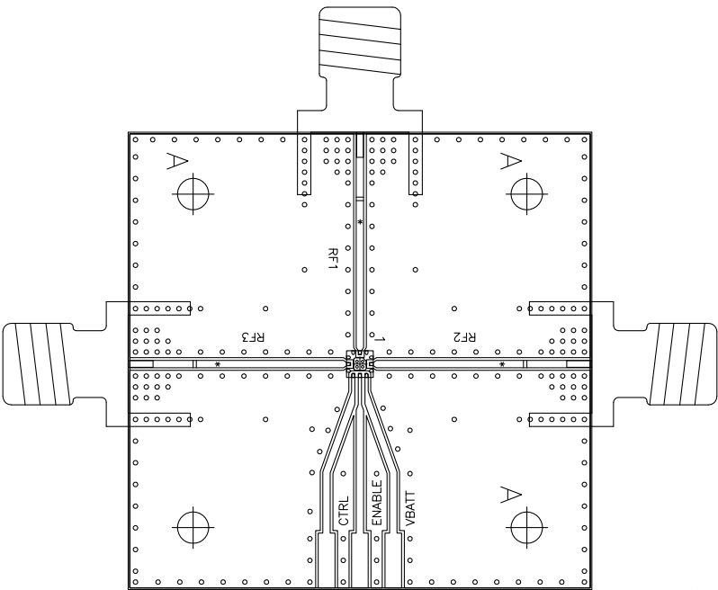
Figure 7. SKYA21003 Evaluation Board Assembly Diagram
