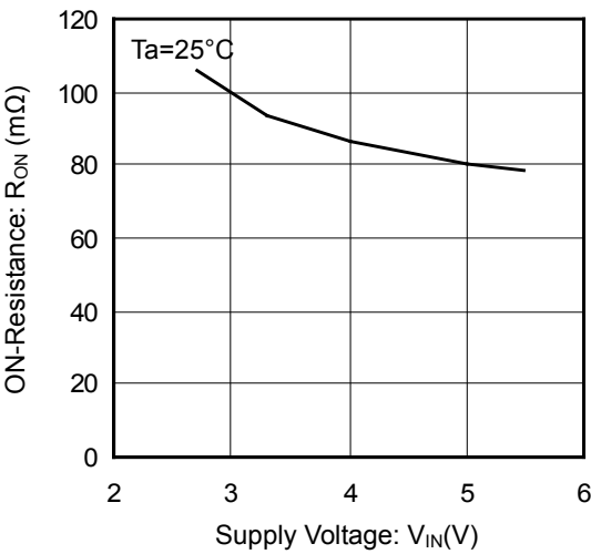
Figure 12. ON-Resistance vs Supply Voltage
