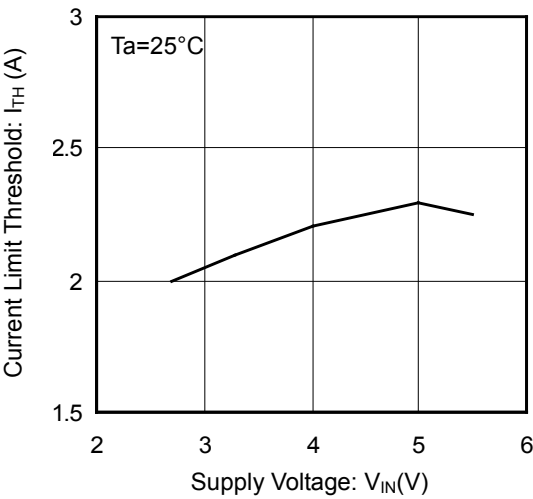
Figure 14. Current Limit Threshold vs Supply Voltage
