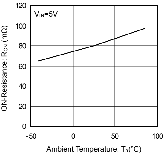
Figure 13. ON-Resistance vs Ambient Temperature
