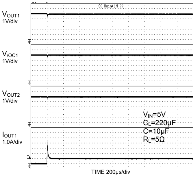
Figure 33. Inrush Current (BD2062FJ)
