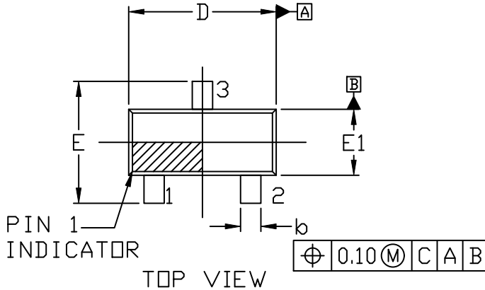
SOT23-3L CASE 318AB ISSUE A
