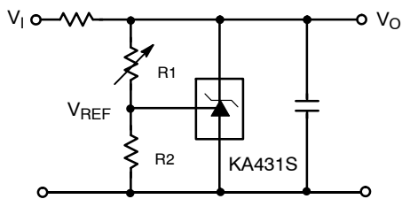
Figure 6. Shunt Regulator
