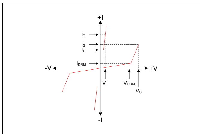
Figure 1. V-I Characteristics
