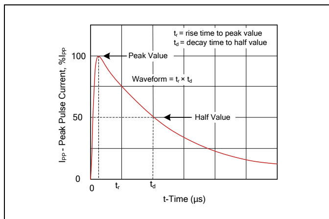
Figure 2. t_r \times t_d Pulse Wave-form
