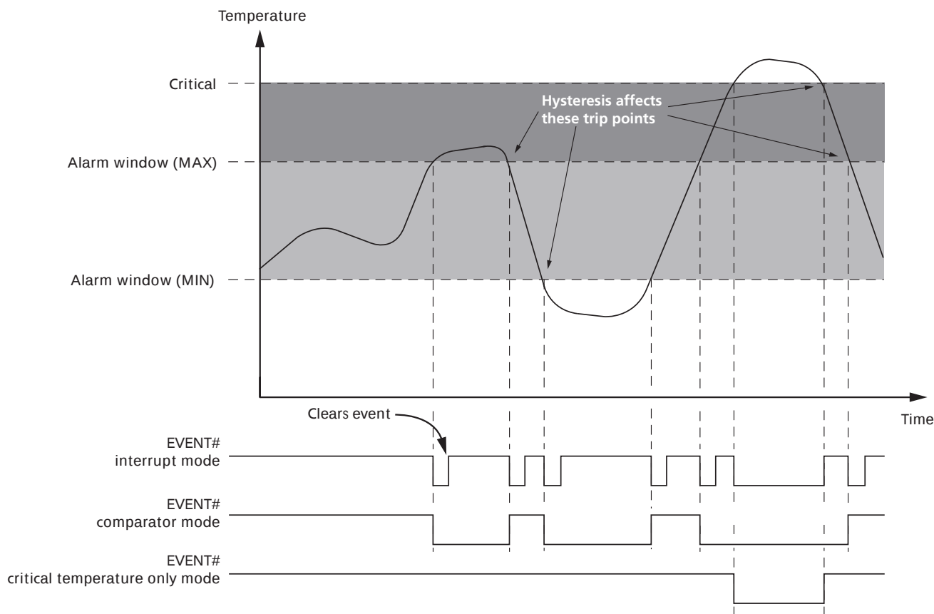
Figure 3: EVENT# Pin Functionality
