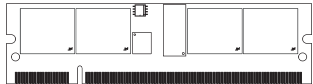
Figure 1: 200-Pin VLP SORDIMM (ATCA Compatible)
