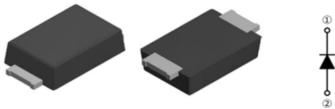
SOD-128
