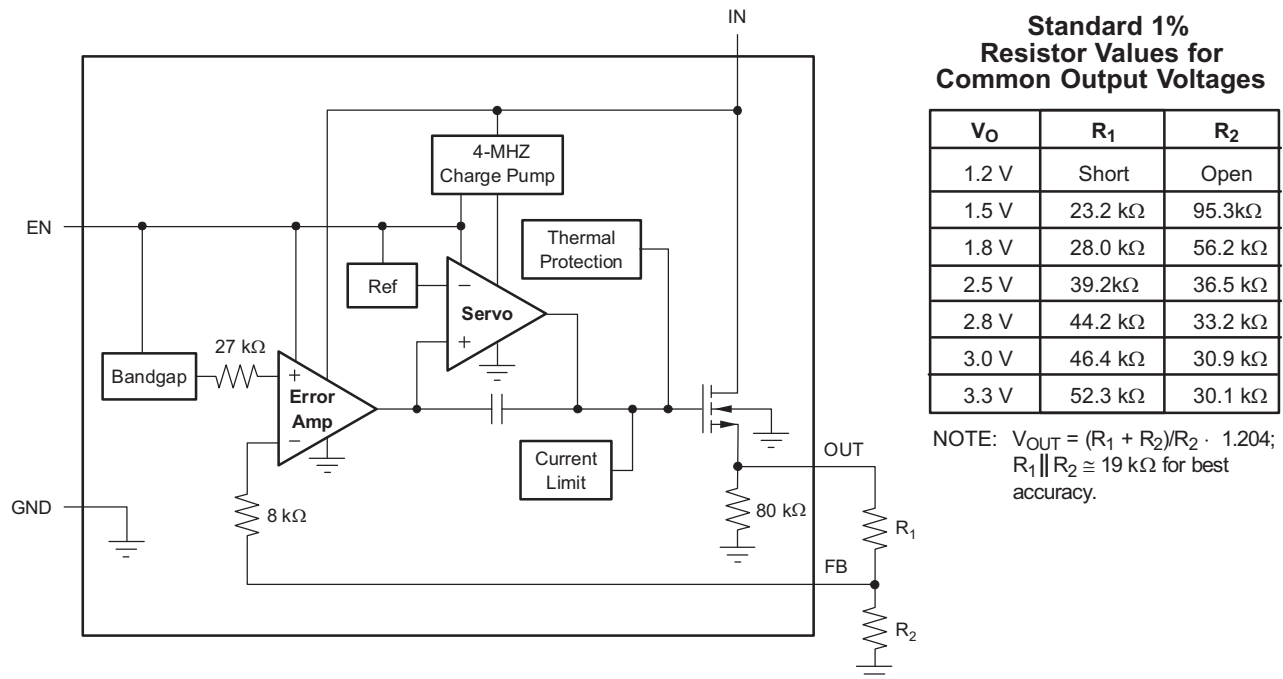
Figure 30. Adjustable-Voltage Version
