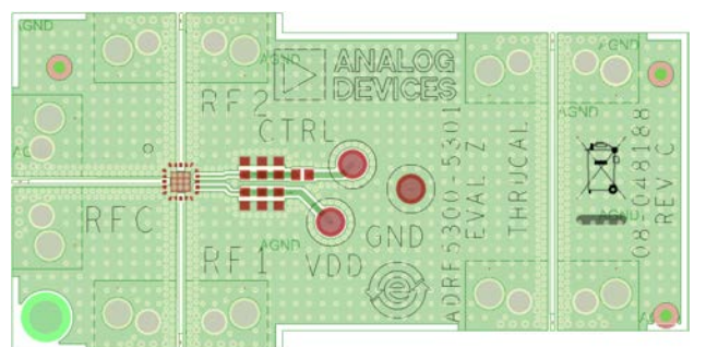
Figure 2. ADRF5300-EVALZ Layout, Top View
