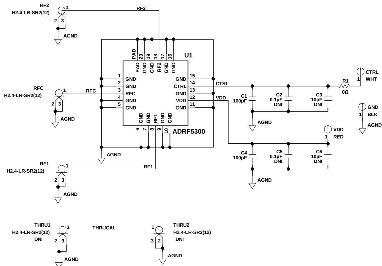
Figure 5. ADRF5300-EVALZ Schematic
